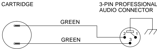
INTERNAL CONNECTIONS
