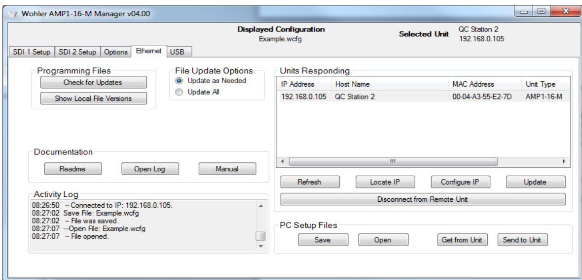
Figure 3–3 AMP1-16-M Manager Ethernet Screen
