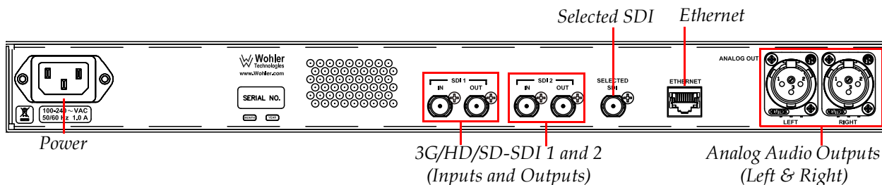
Figure 1–2 Rear Panel Layout
