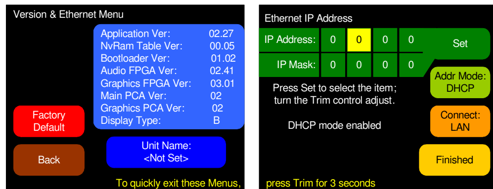
Figure 4–8 Versions and Ethernet Menu
