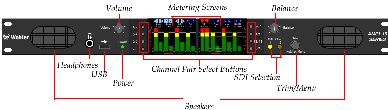
Figure 1-1 Front Panel Layout
