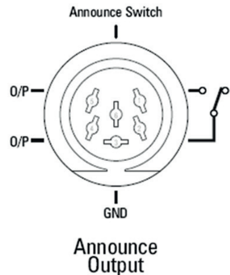
Figure 10: Rear 6-pin DIN socket
