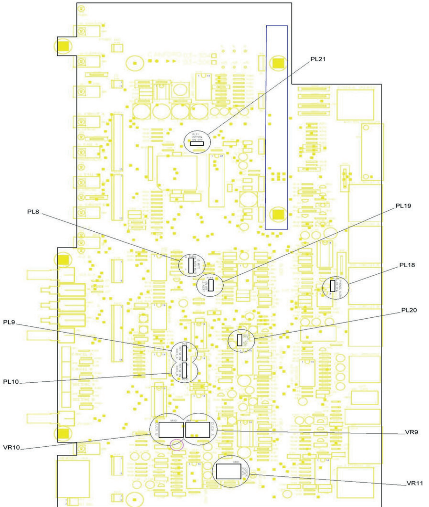
Figure 14: Internal View Of MS741 Main PCB layout
