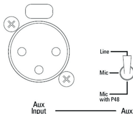
Figure 8: Rear auxiliary input XLR3
