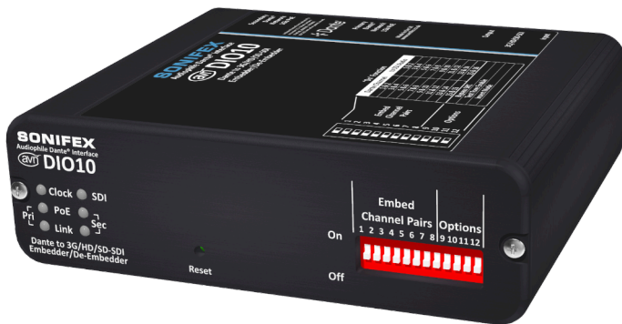
Fig 1-5: AVN-DIO Front Iso View Shown without Accessories
