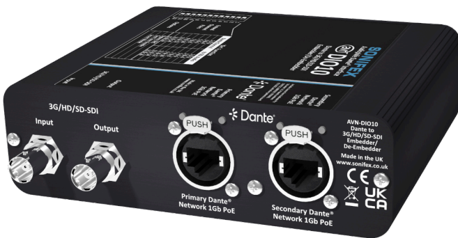
Fig 1-6: AVN-DIO Rear Iso View Shown without Accessories
