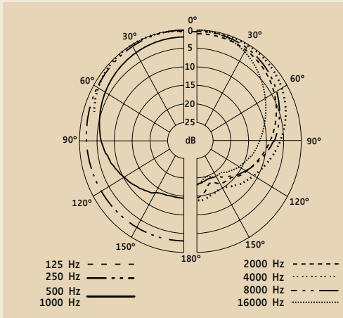
Polar pattern
