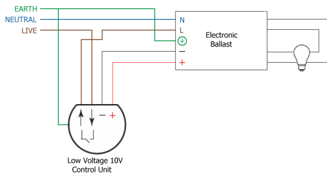
Figure 1 Low Voltage Control Unit set up
