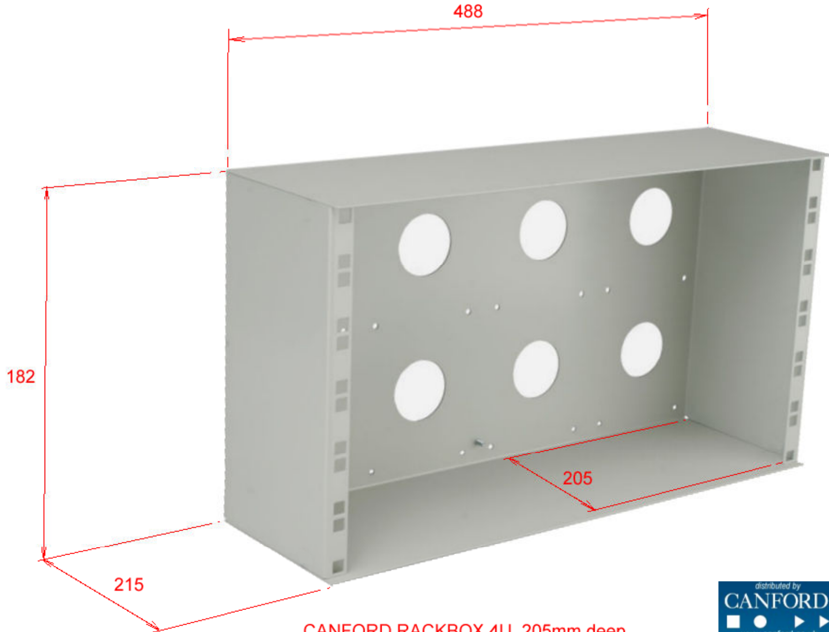
CANFORD RACKBOX 4U, 205mm deep
