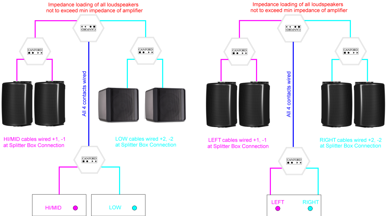
Low Impedance Bi-Amp Application
