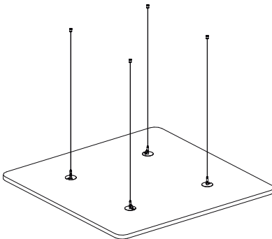
Multiple Point Fixing System
