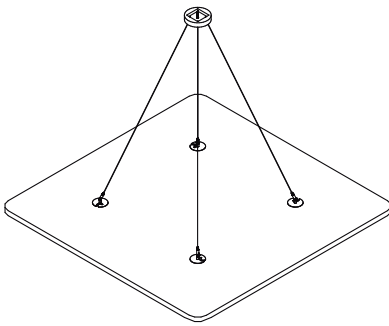
Single Point Fixing System
